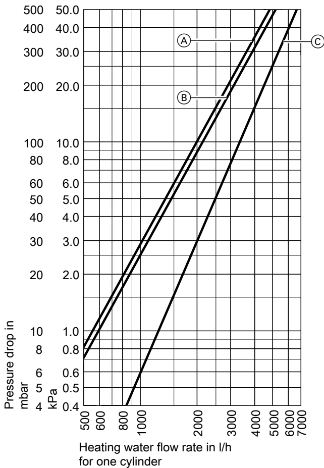
Pressure drop on the heating water side
