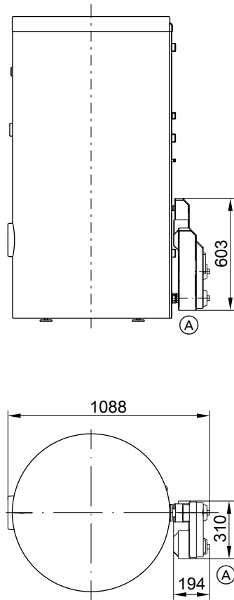
Ⓐ Solar heat exchanger set
