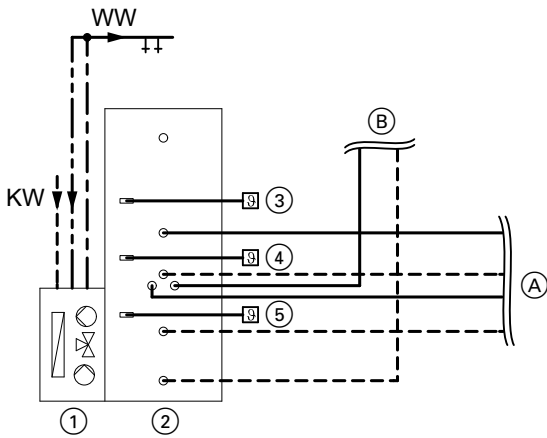
Hydraulic scheme with Vitocell 120-E, type SVW, 600 l
