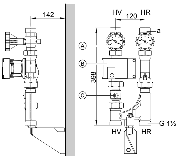
Wall mounted, diagram without thermal insulation
