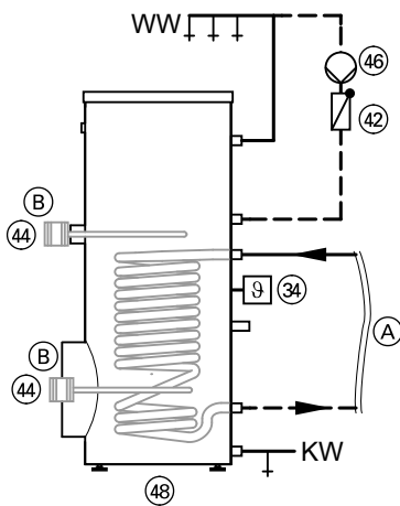
Vitocell 100-V, type CVWA
