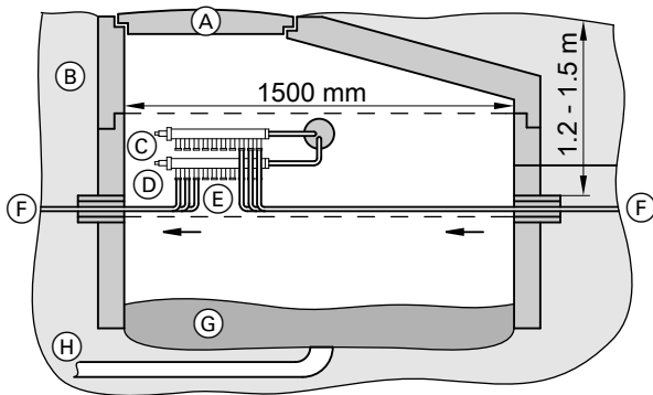
Example of a common duct
