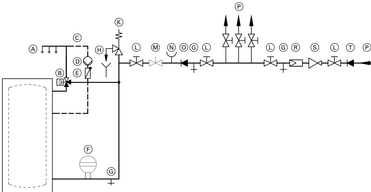
Example with Vitocell 100-V, type CVWA
