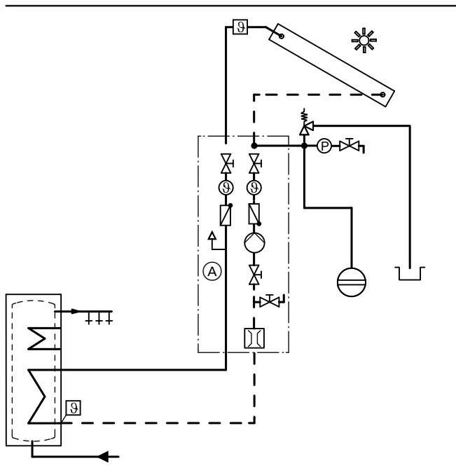
Ⓐ Air vent valve, built into Solar-Divicon
