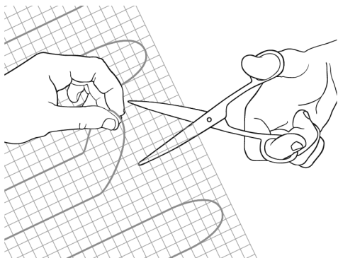
Fig. 19 Correct cutting
