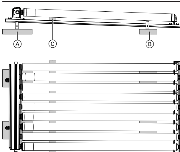
Vitosol 200-TM, type SPEA
