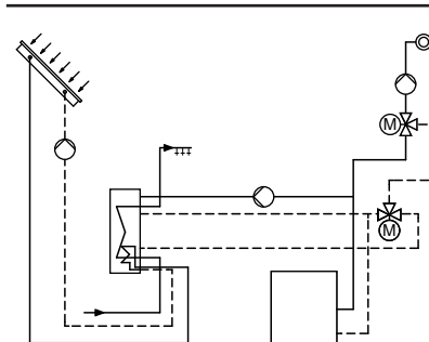
System with Vitocell-M heating water buffer cylinder
