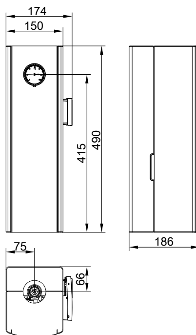
Solar pump assembly
