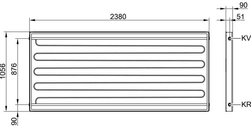
Type SH2F
