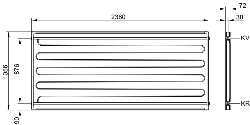
Type SH1F/SH1B
