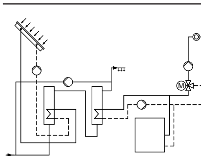
System with 2 mono mode DHW cylinders
