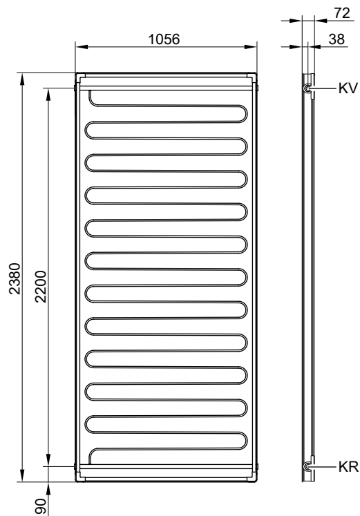
Type SV1F/SV1B
