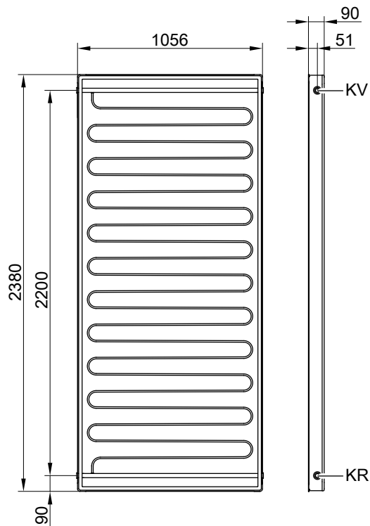
Type SV2F/SV2D
