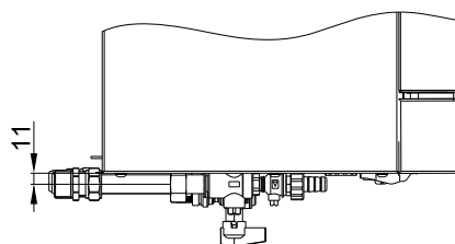
Flush mounting
