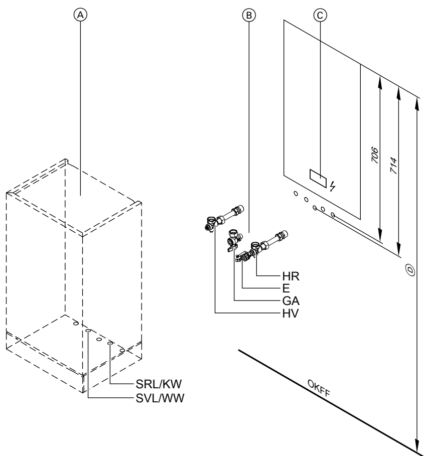
Shown: Connection accessories for Vitodens 100-W gas condensing system boiler
